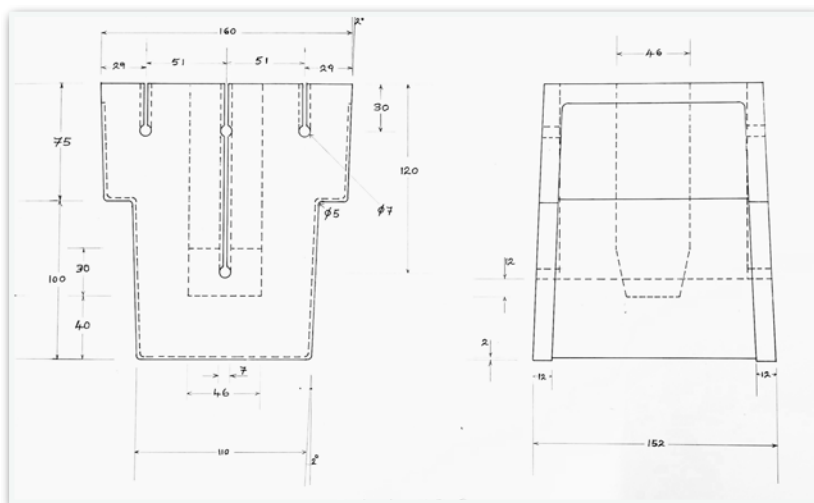
Polystyrene Stop End previously used by client
